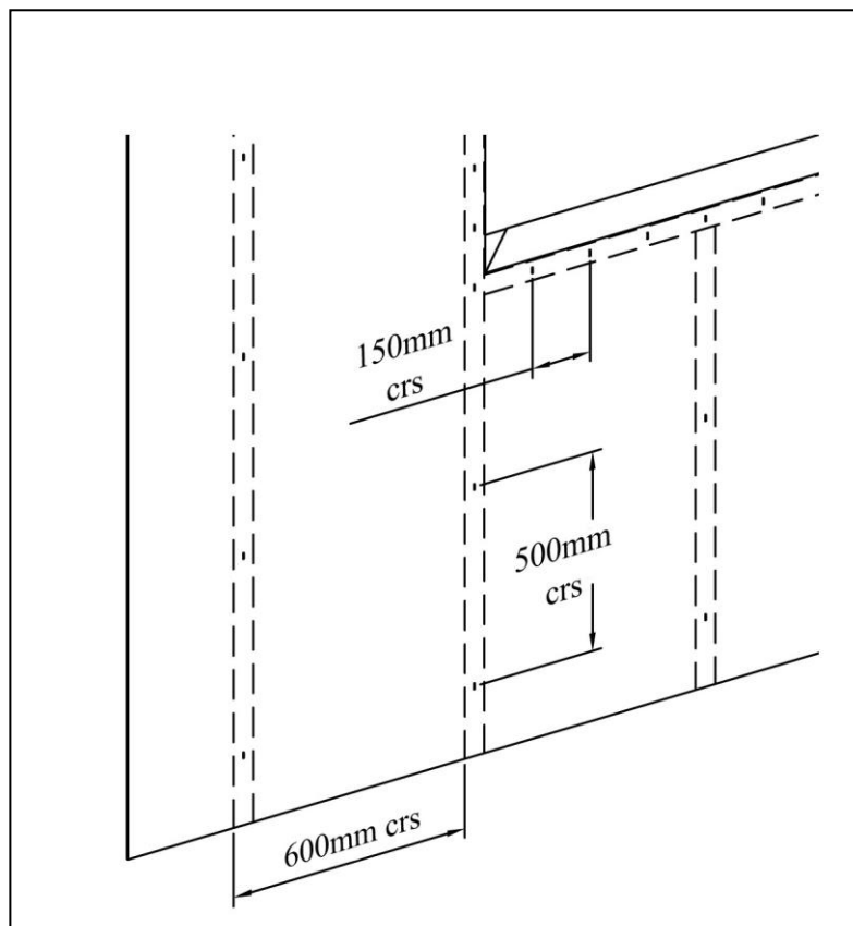
Figure 3: Drawing indicating fixing in factory / on site
