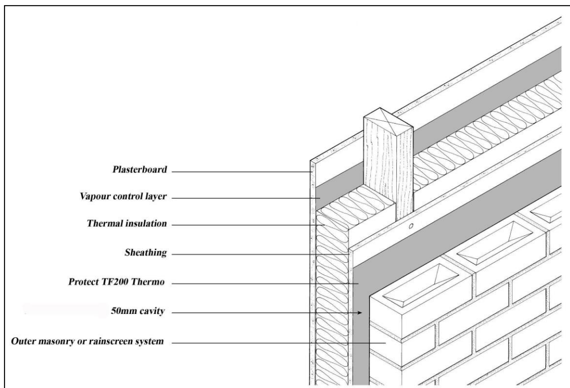
Figure 1: Timber Frame Wall with Protect TF200 Thermo
