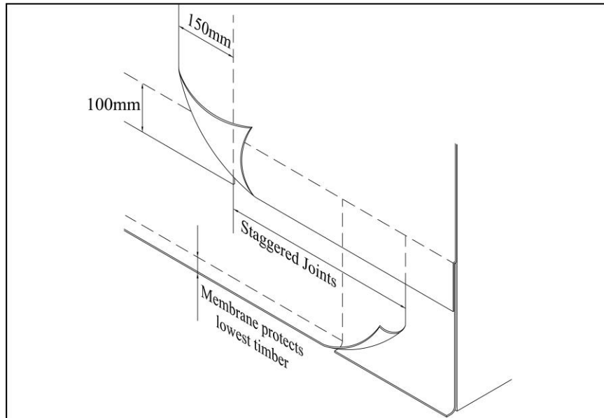
Figure 3: Drawing indicating fixing in factory / on site
